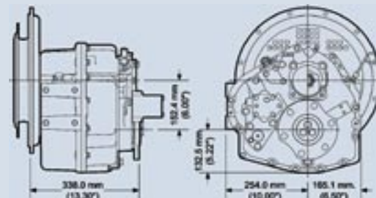
MG-5065 SC (SHALLOW CASE)
