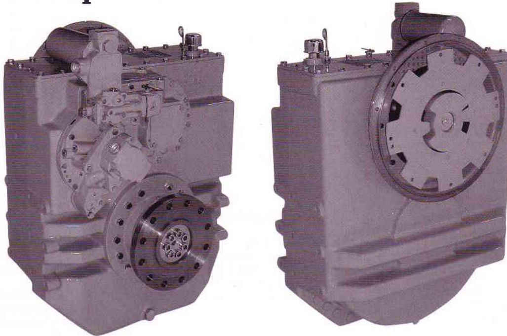
MG-5222DC shown with standard equipment plus optional trolling valve
